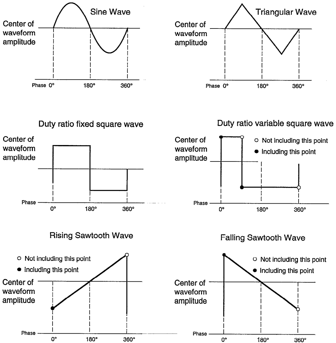
Figure 3-8. Definition of Phase of each Waveform
